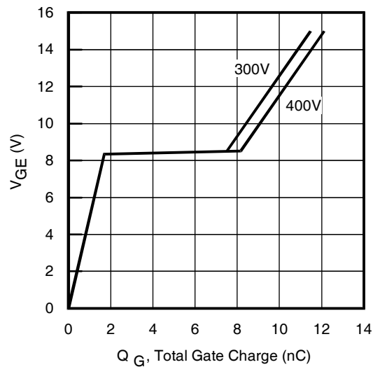
Fig. 23 - Typical Gate Charge vs. V_{GE} I_{CE} = 4.0A ; L = 3150\mu\text{H}
